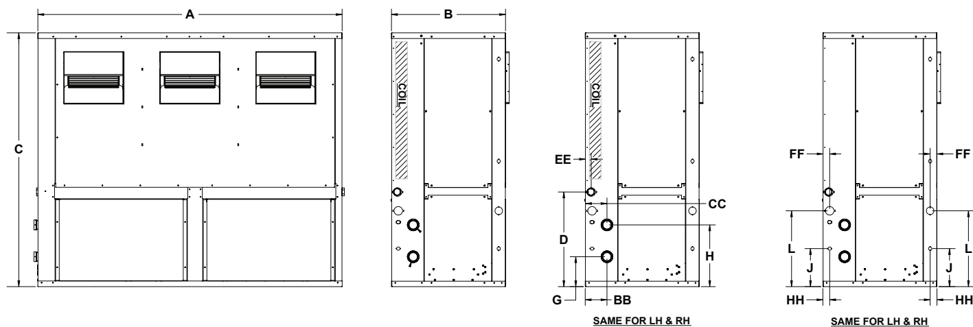
Figure 19: WSLV Unit Dimensions
