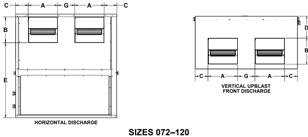
Figure 20: WSLV Discharge Air Dimensions
