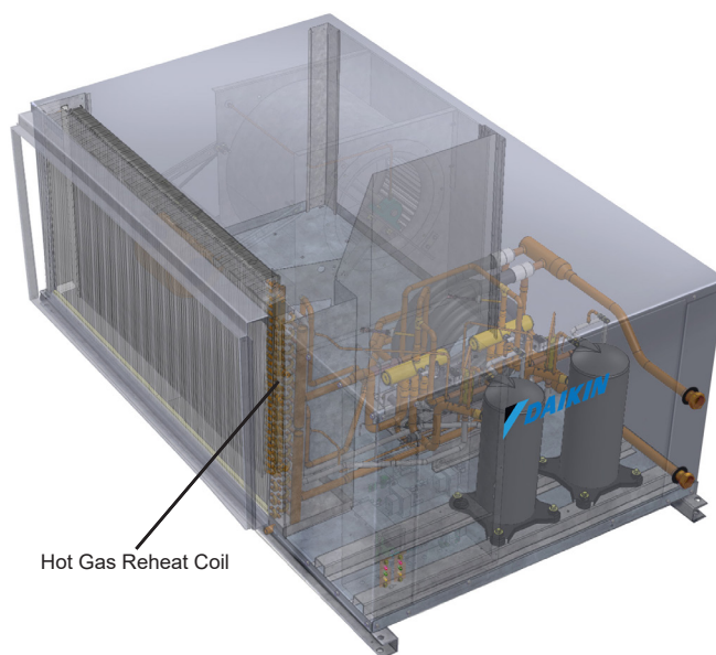
Figure 1: WSLH Unit with Hot Gas Reheat (HGRH)
