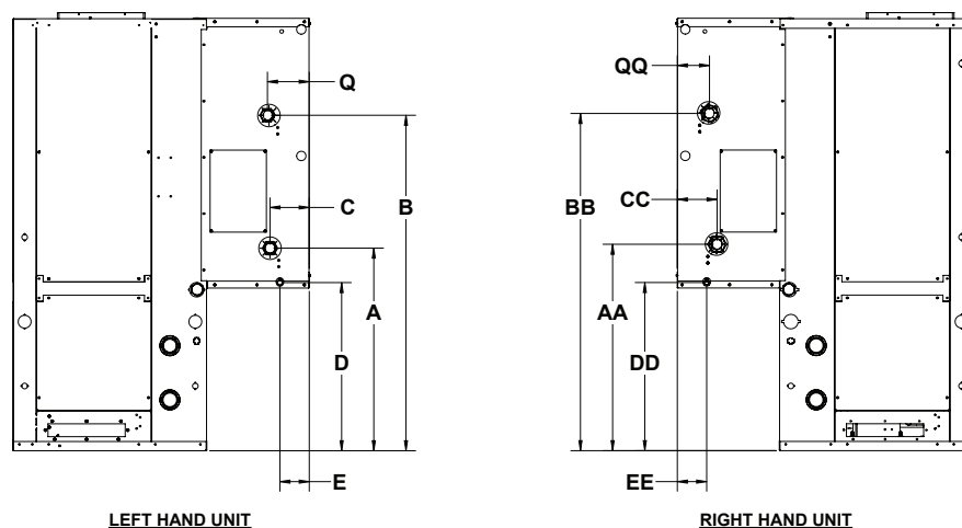
Figure 21: WSLV Unit Dimensions - Economizer/Hydronic Heat Connections & Condensate Drain
